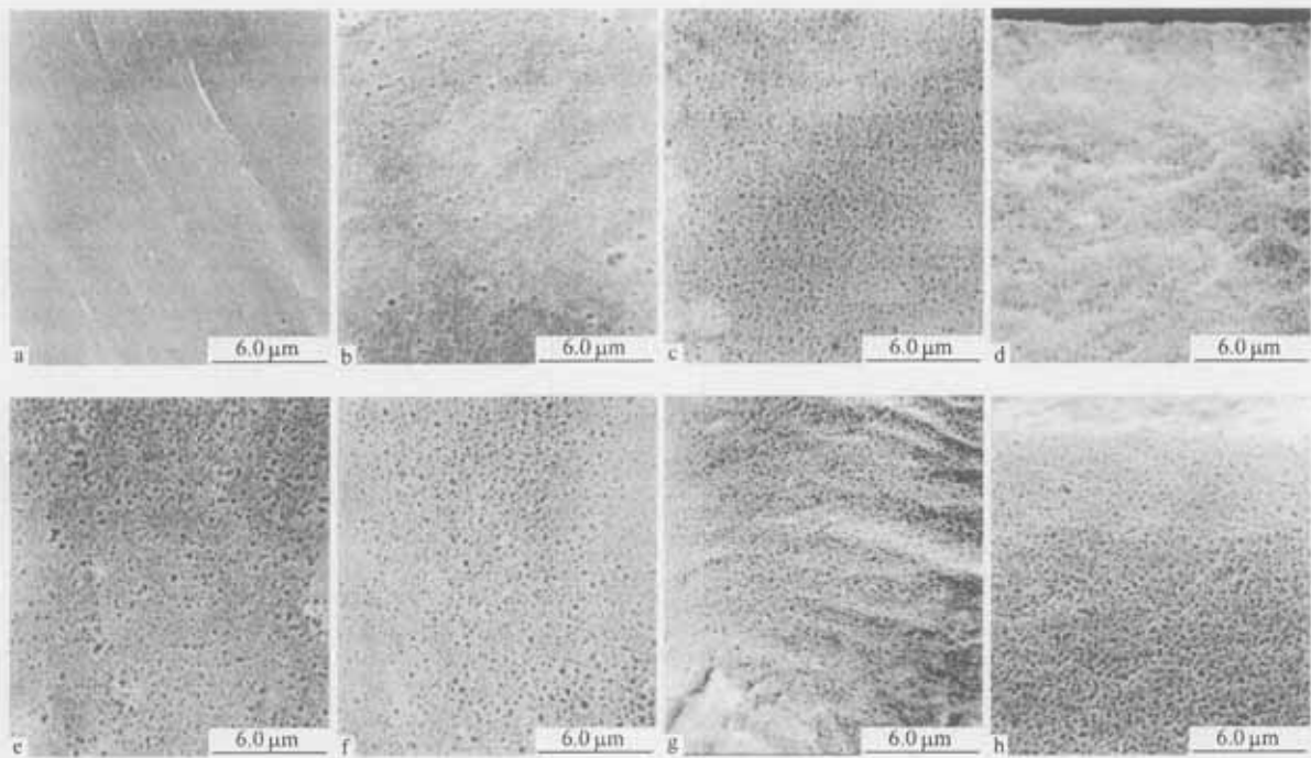
Fig. 5 SEM micrographs of cross-section for pre-hydrolyzed and post-hydrolyzed cellulose acetate membranes a) CA1; b) CA2; c) CA3; d) CA4; e) CA5; f) CA4-2; g) CA4-8; h) CA4-24
