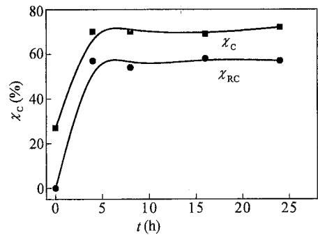
Fig. 4 Dependence of crystallinities of hydrolyzed membranes on hydrolysis time; \chi_c — total crystallinity, \chi_{RC} — crystallinity of cellulose II
