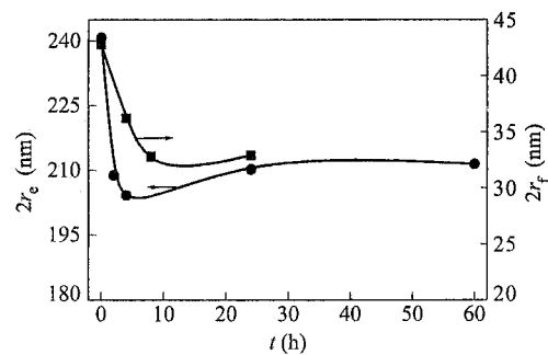
Fig. 6 Dependence of the porous sizes of pre-hydrolyzed and post-hydrolyzed CA4 on hydrolysis time by dilute alkali ● Measured by SEM imaging analysis system ■ Measured by osmometry
